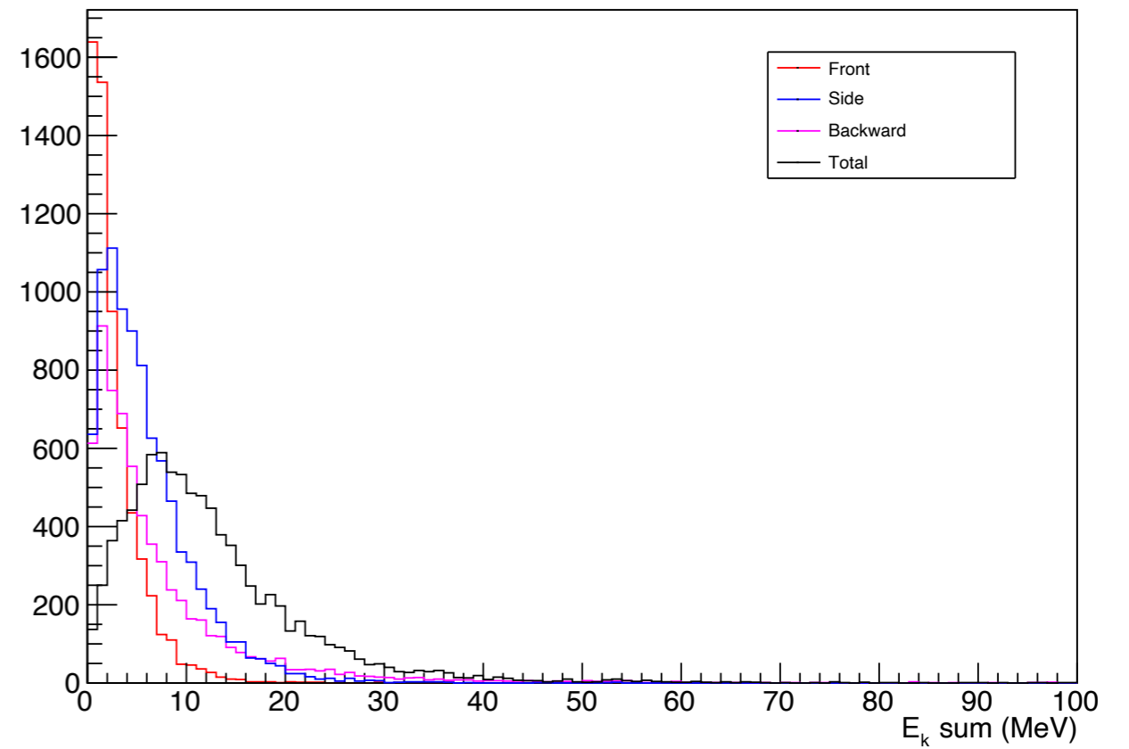
FTFP_BERT
