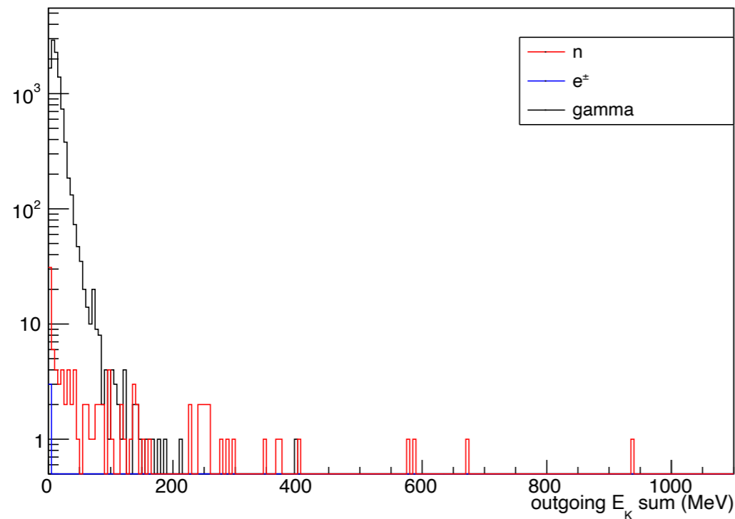
FTFP BERT
