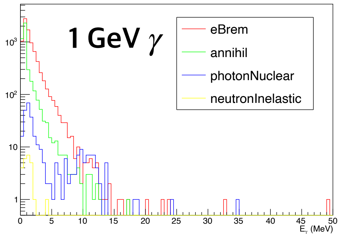
Backsplash \gamma creator process
