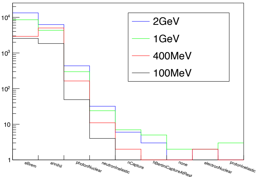
Backsplash \gamma creator process
