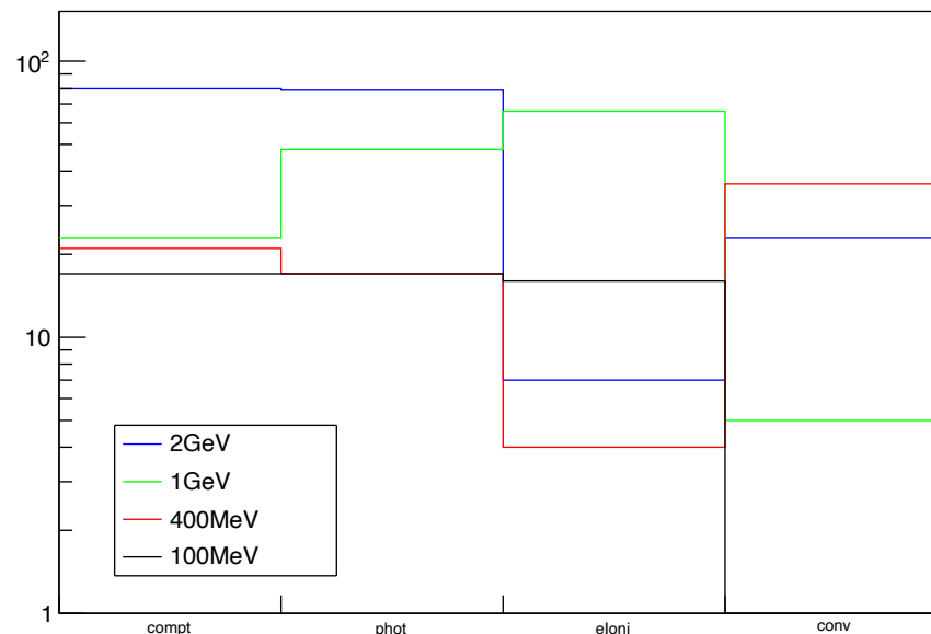
Backsplash e^- creator process
