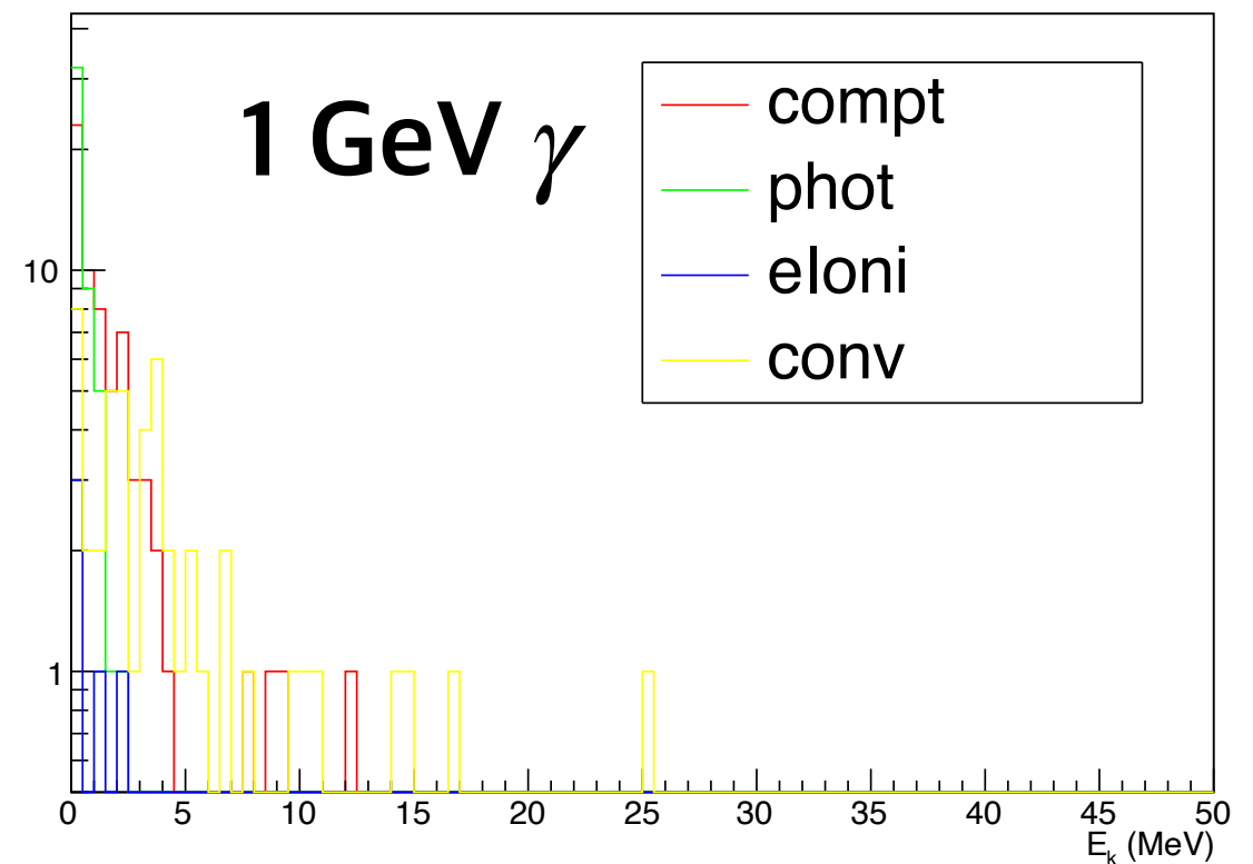
Backsplash e^\pm creator process
