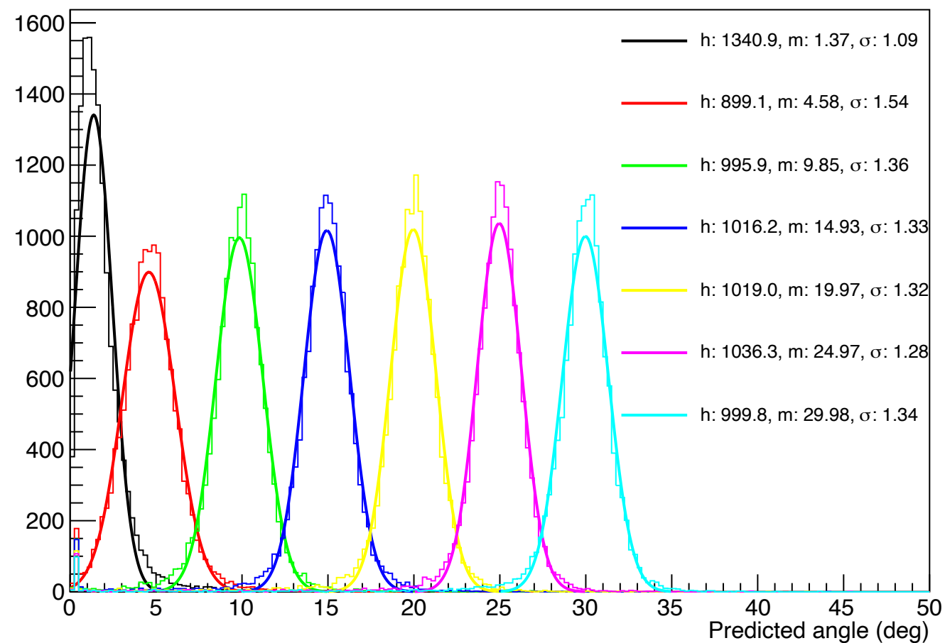
Ecut 0 MeV
