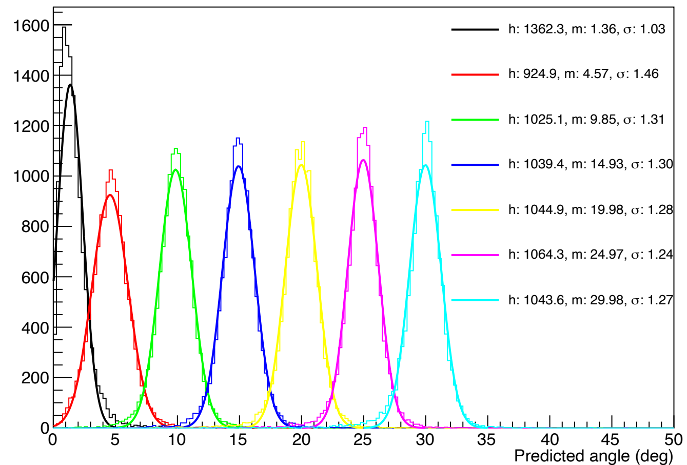
Ecut 10 MeV
