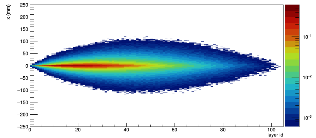
Lead 1mm + Scint 5mm
