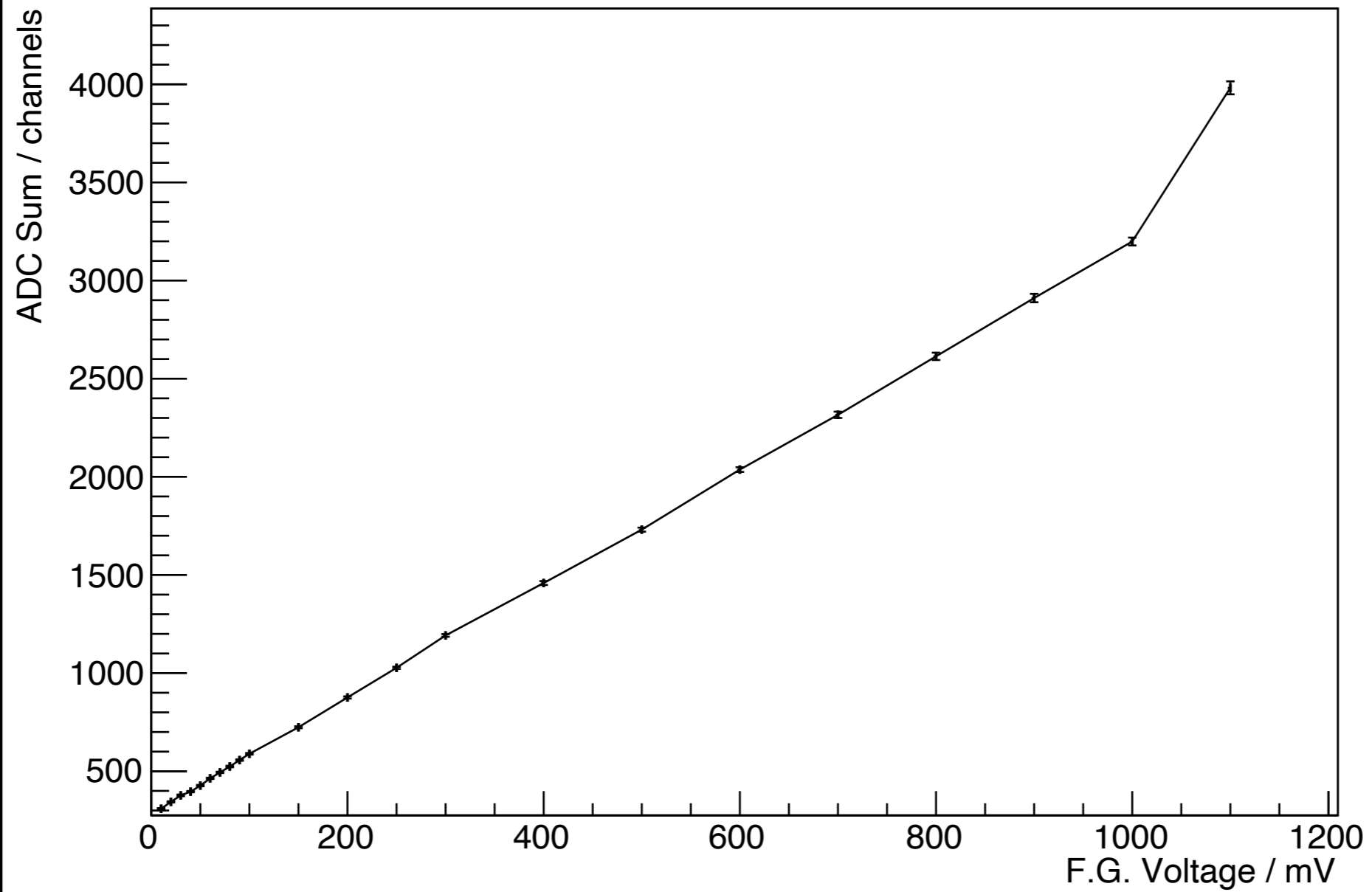
F.G. Voltage vs. ADC Sum
