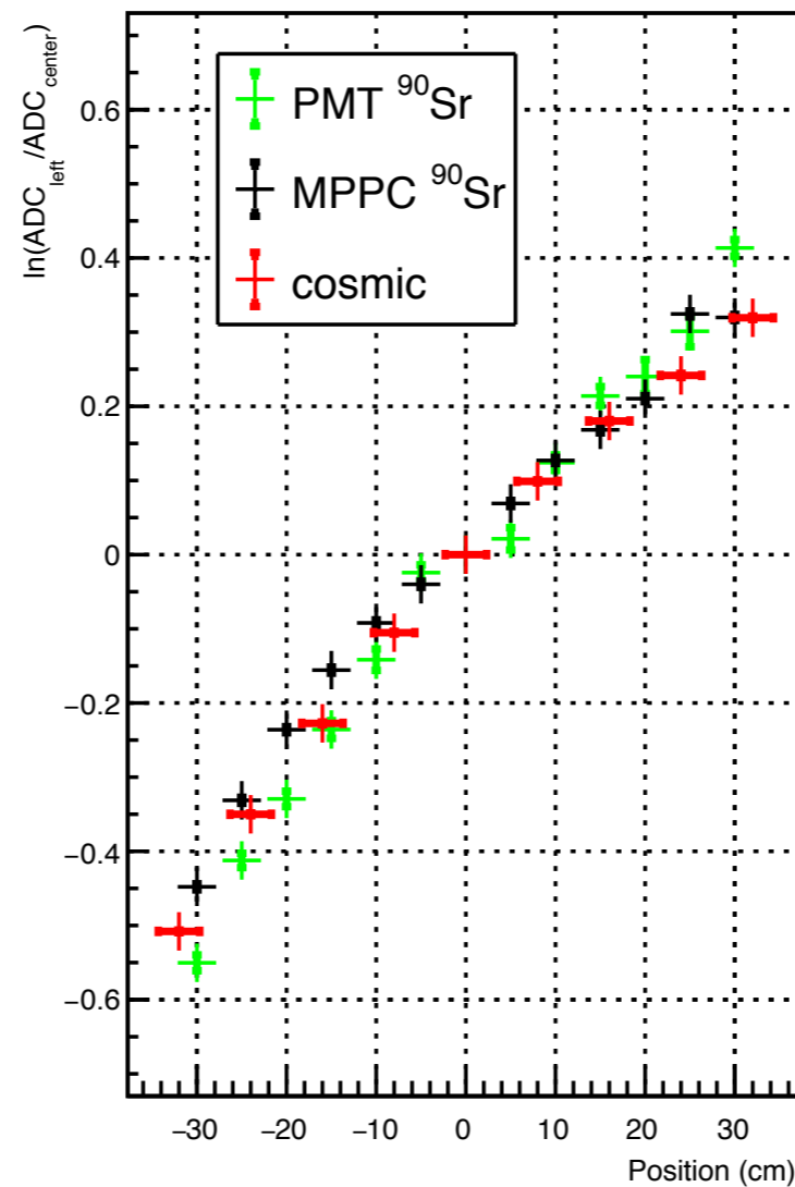
Attenuation length(left)
