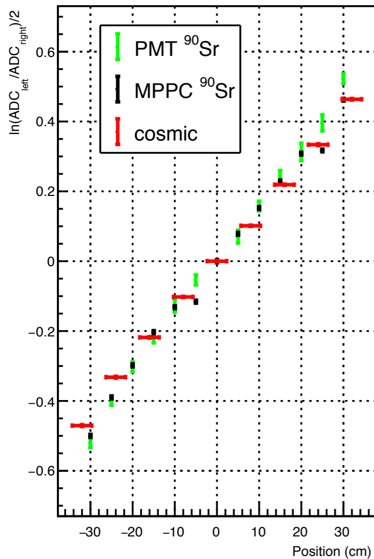
Attenuation length
