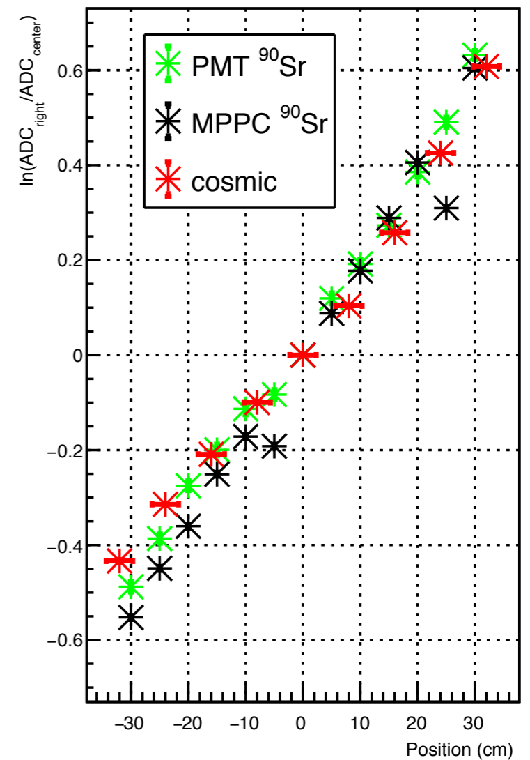
Attenuation length(right)
