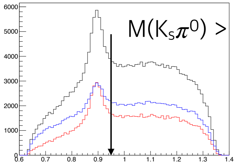
M(K s π 0 )
