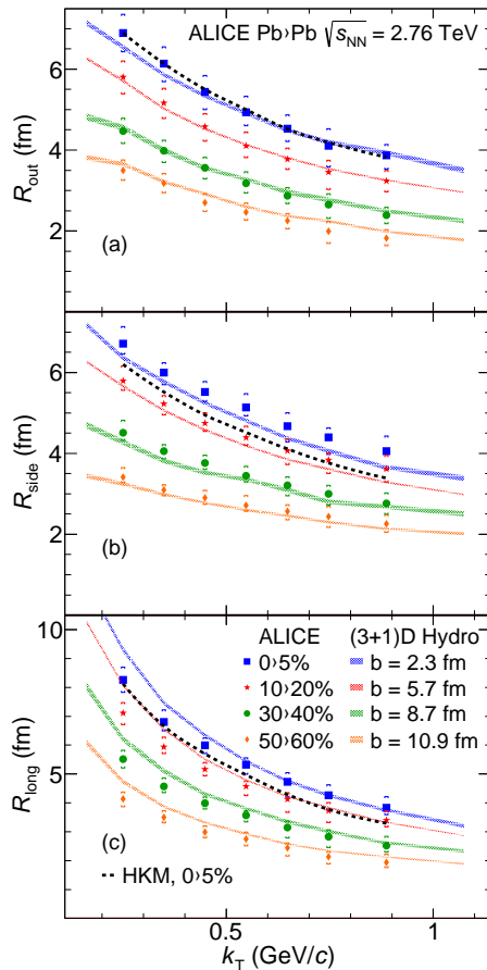
Figure 2. Comparison of femtoscopic radii, as a function of pair transverse momentum, with the calculation from the Therminator and 3+1D hydro model [2], for four centralities and with the HKM model [3] for the central data. Closed symbols are experimental data, bands and dashed lines are the model calculations. Figure from [4]
