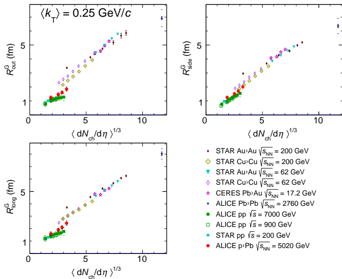
Figure 1. Comparison of femtosopic radii (Gaussian), as a function of the measured charged-particle multiplicity, for various collision systems and energies. Figure from [5]
