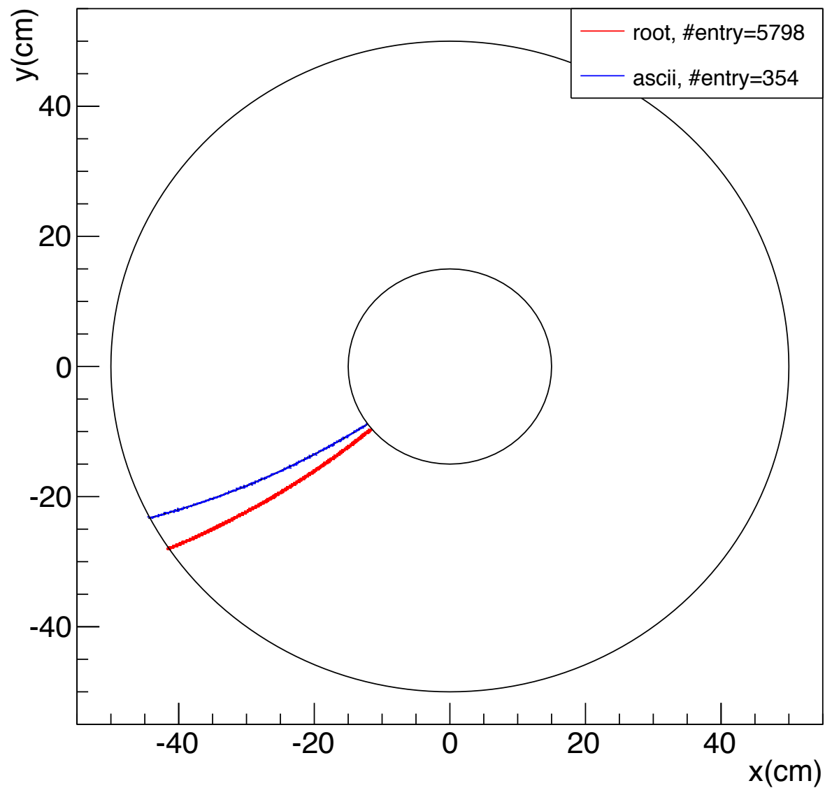
Proton, 0.2 GeV, \phi = 220^\circ , \theta = 70^\circ
