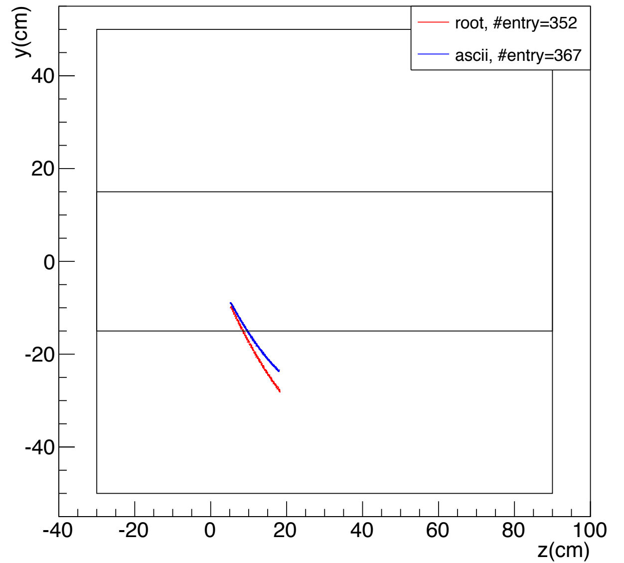
Proton, 0.2 GeV, \phi = 220^\circ , \theta = 70^\circ
